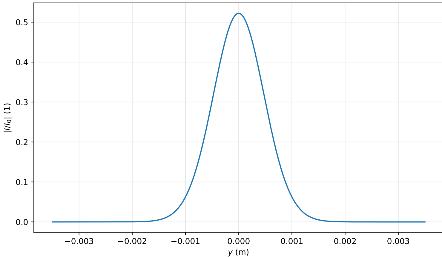
Intensity profile I(x=0, y, z=2.070)/I_0 , \text{Pin}=0.1\text{Pcr} , artificial time
